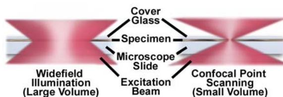
Figure 4. Widefield versus confocal microscopy illumination volumes, demonstrating the difference in size between point scanning and widefield excitation light beams.
