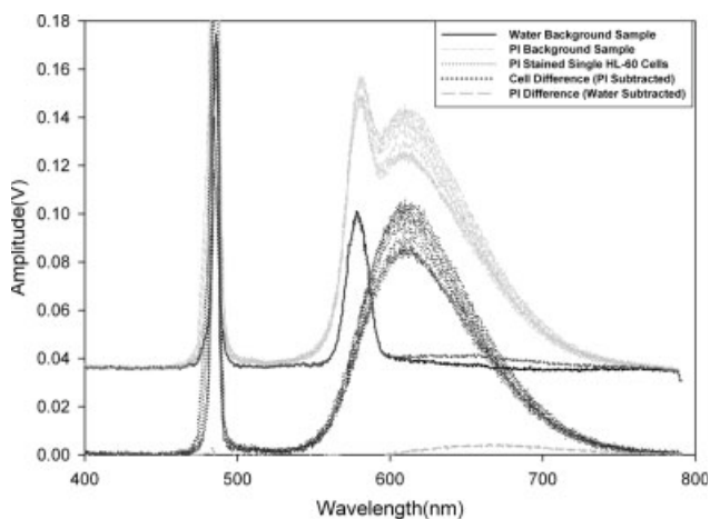
FIG. 6. Spectra of fifteen individual PI-stained HL-60 cells excited with a 488 nm laser. The black line corresponds to the background spectra with only water in the sample stream. The dotted line indicates the background spectrum of PI in the sample stream in the absence of cells, the light gray short dashed lines correspond to individual PI-stained cells, and the dark gray dashed lines are the difference of each cell spectrum and the PI background. The light gray line is the difference of PI-only sample from the water background. The leftmost peak in the scattered laser light, the narrow peak near the center, most visible in the two background spectra, corresponds to the Raman scatter due to the stretching mode of water, and the broad peak corresponds to PI fluorescence. The rightmost peak in the background-subtracted PI-only spectrum corresponds to unbound PI, while the narrower and higher peak visible in the background-subtracted sample spectra corresponds to bound PI.
