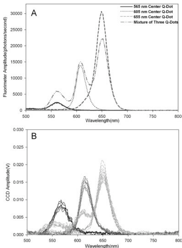
FIG. 5. Graph of fluorescence spectra from biotin microspheres labeled with three different types of streptavidin-coated quantum dots with 488 nm, 100 mW excitation. Each quantum dot had a center fluorescence at the specified wavelength. (A) Spectra from samples of quantum dot-labeled microspheres measured with a PTI fluorimeter. (B) Ten individual spectra from single microspheres measured with the spectral flow cytometer; A background spectra from DI water has been subtracted from each single bead spectrum.
