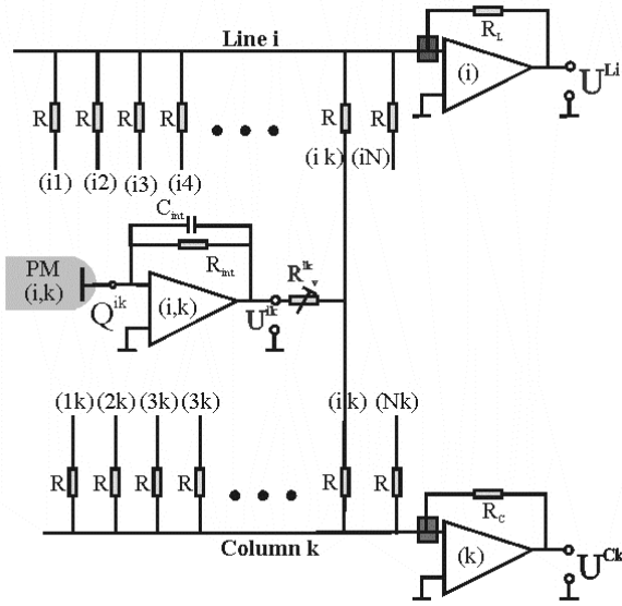
Fig. 4 Current distributions into line and column SUM amplifier.
